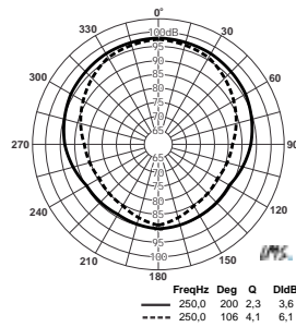
FT212 - SPL POLAR DIAGRAM (Field Measurement - 6.1 meters (20 feet))
